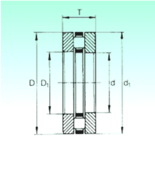
81206TN Bearing 2D drawings and 3D CAD models
